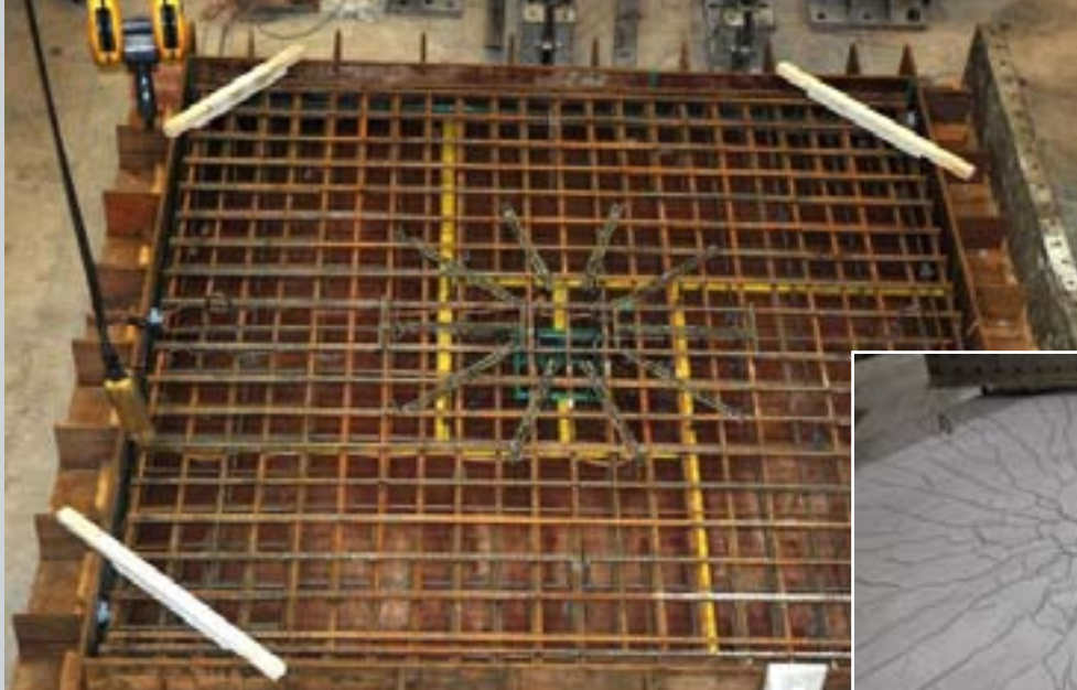
Figure 3 - LinkStudPSR Testing
